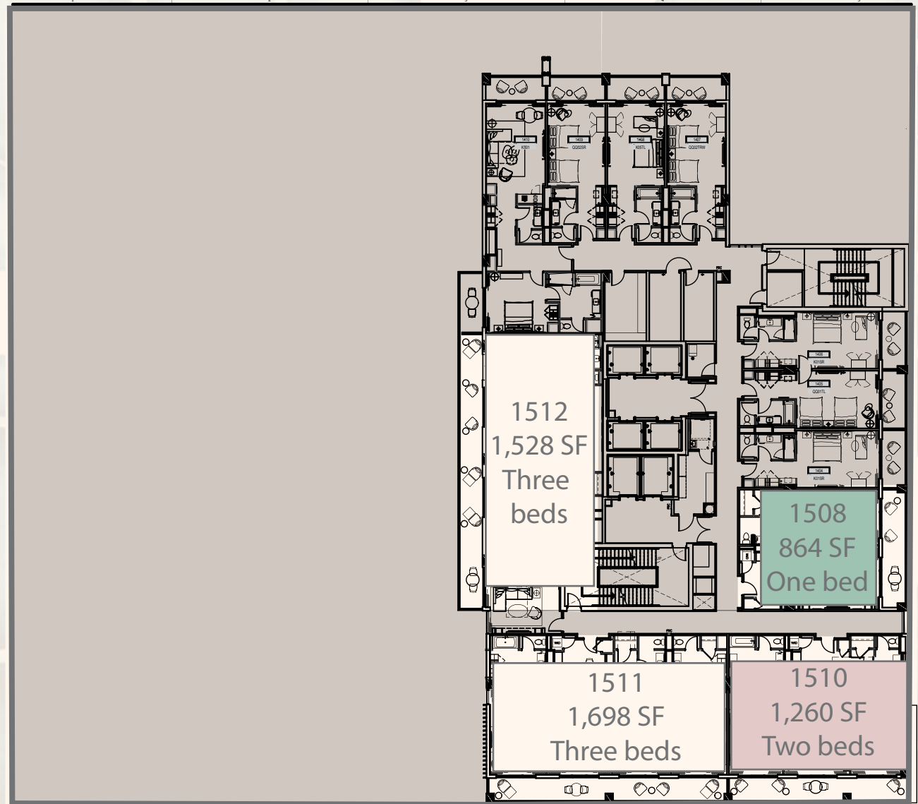
15TH FLOOR - KEY PLAN
