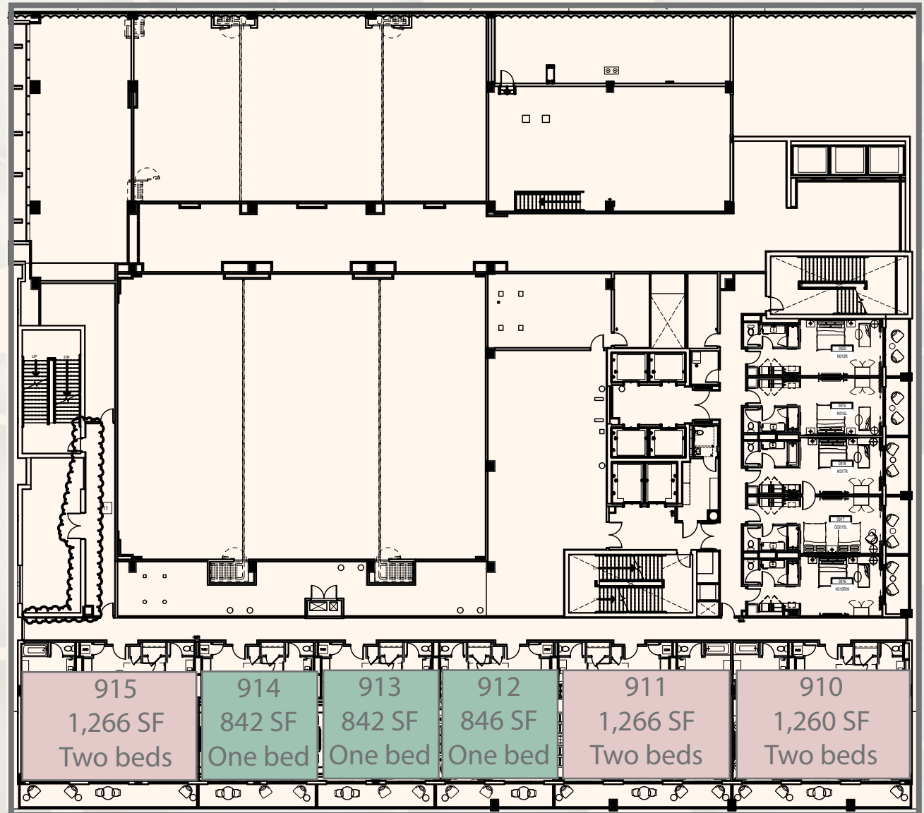
9TH FLOOR - KEY PLAN
